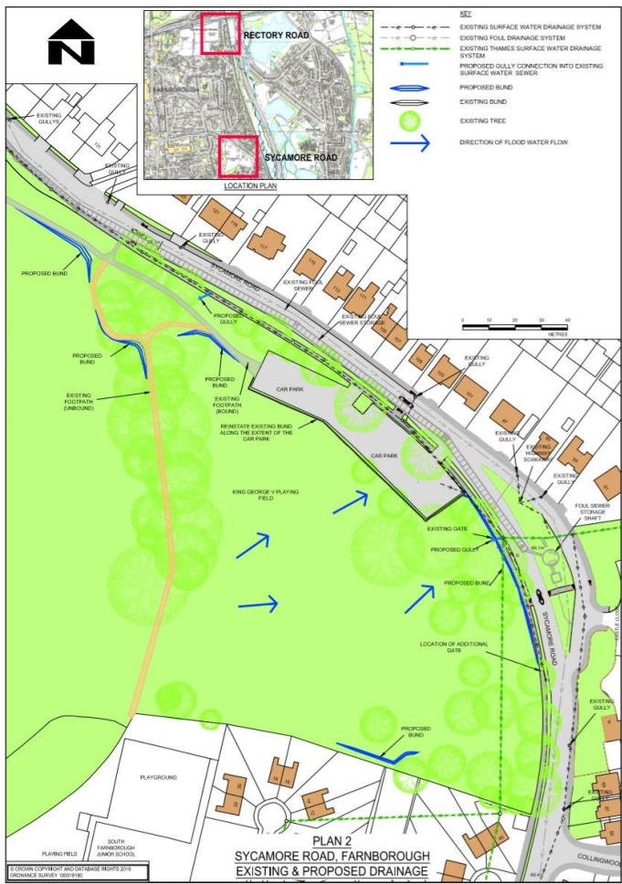
2: Sycamore Road existing and proposed drainage
